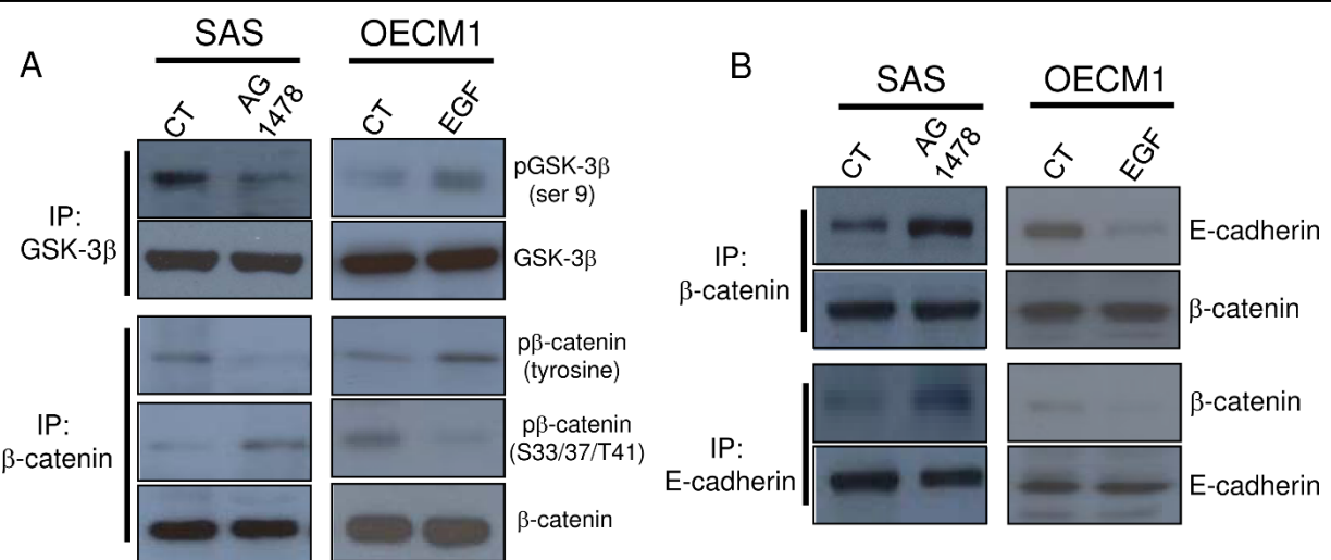
Figure 2 Effects of EGFR signal on the phosphorylation and function of \beta -catenin and GSK-3 \beta . (A) AG1478 treatment of SAS cells decreased phosphorylation of GSK-3 \beta (Ser-9) and \beta -catenin (Tyr). EGF treatment of OECM1 cells increased phosphorylation of GSK-3 \beta (Ser-9) and \beta -catenin (Tyr), as determined by immunoprecipitation of GSK-3 \beta or \beta -catenin. (B) In SAS cells, association of E-cadherin and \beta -catenin increased following treatment with AG1478; in OECM1 cells, association of E-cadherin and \beta -catenin decreased following treatment with EGF as determined by immunoprecipitation of E-cadherin or \beta -catenin.
