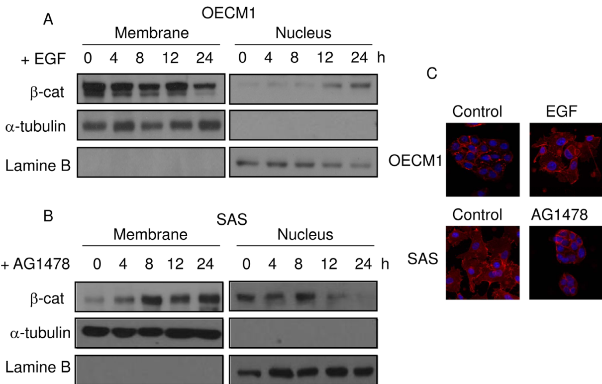
Figure 1 Effect of EGFR on the subcellular distribution of \beta -catenin in oral cancer cell lines. Time-dependent effects of EGF or AG1478 on the subcellular distribution of \beta -catenin in OECM1 (A) and SAS (B) cells. Cancer cells were treated with EGF (100 ng/mL) or AG1478 (20 \mu M/mL) for the indicated time, and \beta -catenin was assayed by Western blotting. (C) Immunocytochemical staining of \beta -catenin in oral cancer cells. EGF treatment of OECM1 cells induced scattering of cancer cells, breakup of cell-cell junctions, and decreased level of membranous \beta -catenin (upper panels). AG1478 treatment of SAS cells led to close cell-to-cell contact and abundant membranous \beta -catenin (lower panels). Immunofluorescence for \beta -catenin (Rhodamine, Red) and the nucleus (Dapi) in cultured cells was performed 24 h following treatment. Cells were permeabilized with 100% methanol, blocked with 1% BSA, and incubated with the antibody for 30 min. A rhodamine conjugated antibody was used as the secondary antibody.
